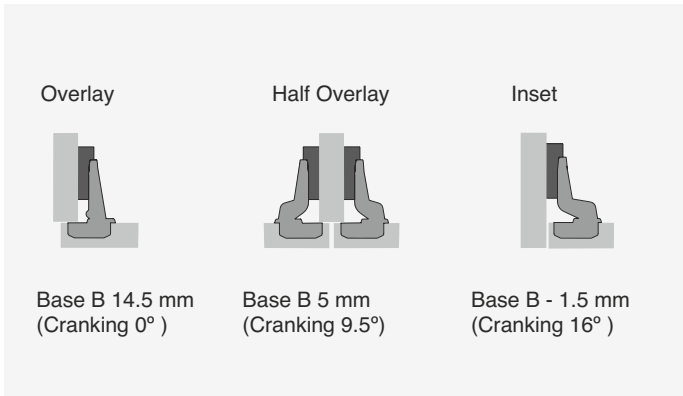
Minimum Reveal Per Door
