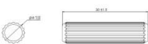
Wooden Dowel 8x30mm
