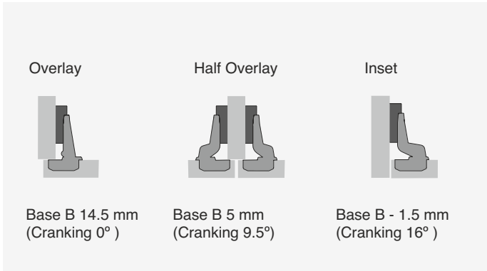
Minimum Reveal Per Door
