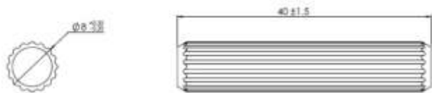
Wooden Dowel 8x40mm
